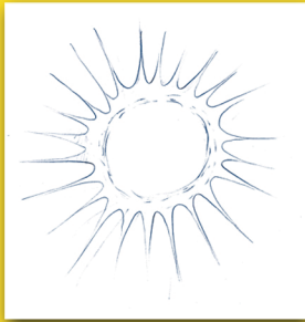
Soleil
